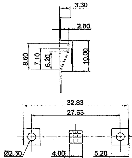
PCB Mounting layout
