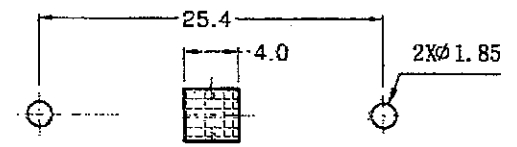
PCB Mounting layout
