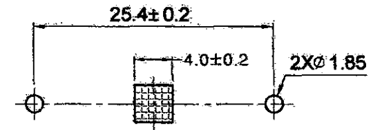
PCB Mounting layout
