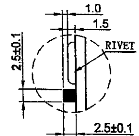
POLARITY PROTECTION DEVICE DETAIL "A" S=1.5
