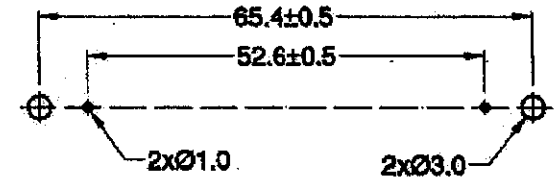
PCB/MOUNTING LAYOUT
