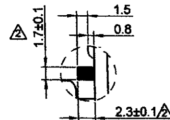
POLARITY PROTECTION DEVICE DETAIL "A" S=2
