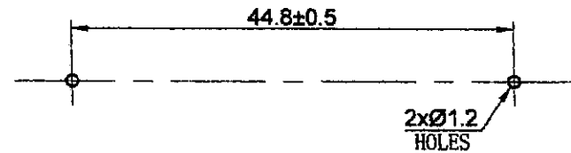
PCB/MOUNTING LAYOUT
