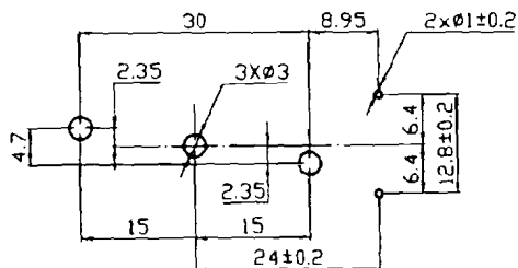
PCB/MOUNTING LAYOUT
