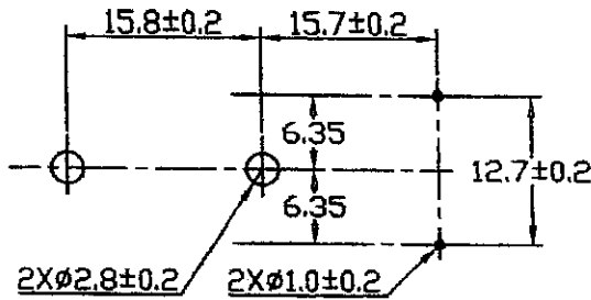
PCB/MOUNTING LAYOUT
