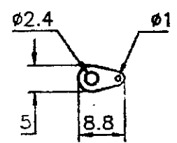
SOLDER TERMINAL
