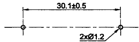
PCB/MOUNTING LAYOUT
