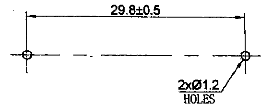
PCB/MOUNTING LAYOUT
