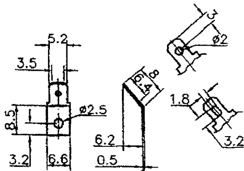
TERMINAL
