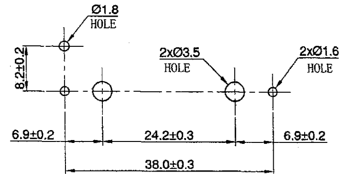
PCB/MOUNTING LAYOUT
