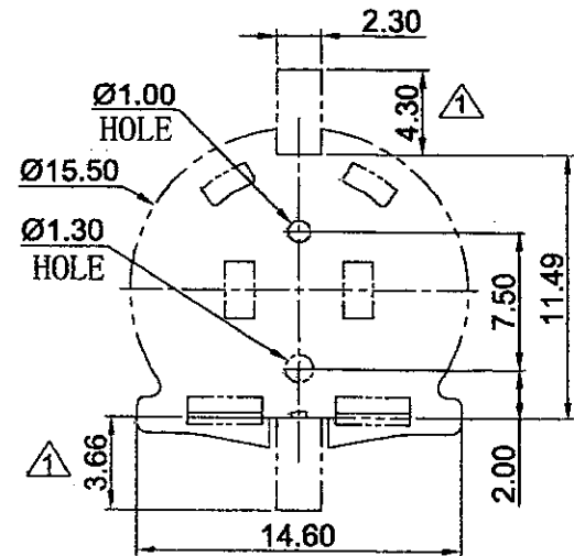
PCB MOUNTING LAYOUT
