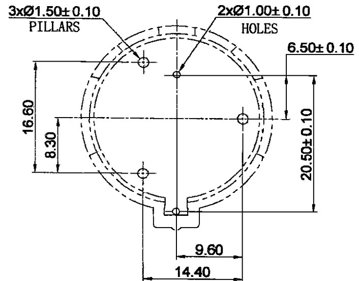
PCB MOUNTING LAYOUT
