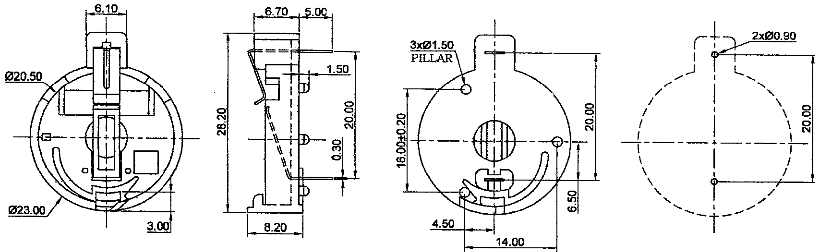
PCB MOUNTING LAYOUT
