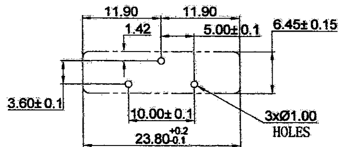
PCB MOUNTING LAYOUT
