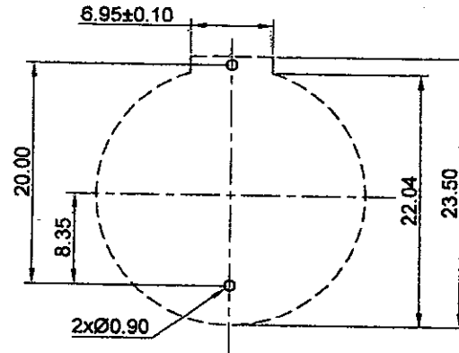
PCB MOUNTING LAYOUT
