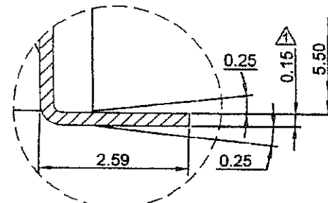
DETAIL "B" S=6
