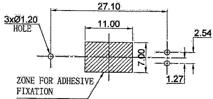
PCB/MOUNTING LAYOUT
