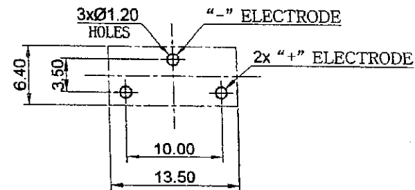
PCB MOUNTING LAYOUT
