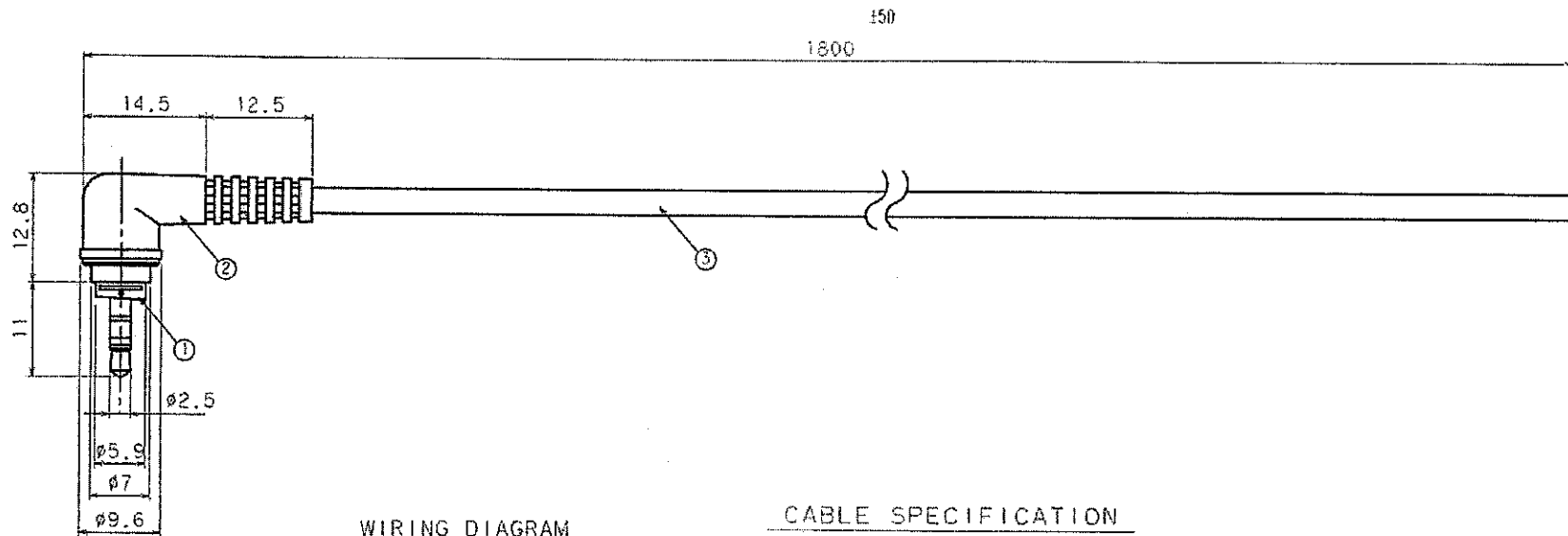
WIRING DIAGRAM
