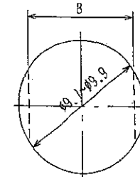
取付板板厚 Thickness of mounting board t=1.0~1.8
