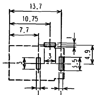
FOOT PRINT(REFERENCE) CIRCUIT
