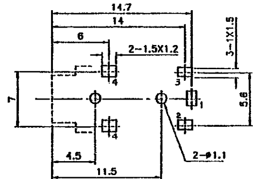
PC BOARD HOLE LAYOUT (VIEW FROM DIRECTION OF INSERTION TO PCB)
