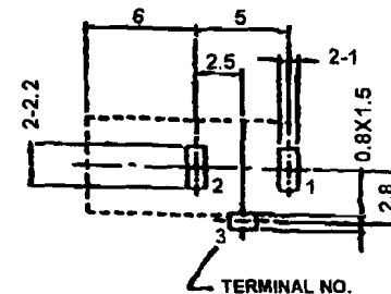
PC BOARD HOLE LAYOUT (UPPER VIEW FROM THE DIRECTION OF INSERTION TO PCB)
