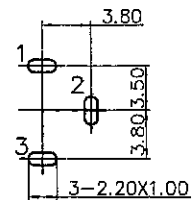
Pin Hole Layout (Jack Bottom View)
