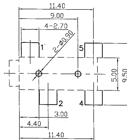
Pin Hole Layout (Jack Bottom View)
