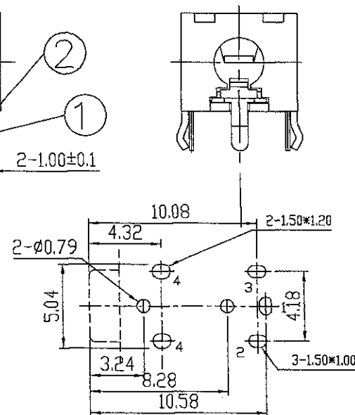
Pin Hole Layout (Jack Bottom View)
