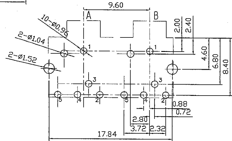
Pin Hole Layout <Jack Bottom View>
