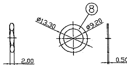
WASHER
