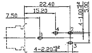
Pin Hole Layout (Jack Bottom View)
