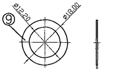
WASHER
