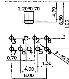
Pin Hole Layout (Jack Bottom View)
