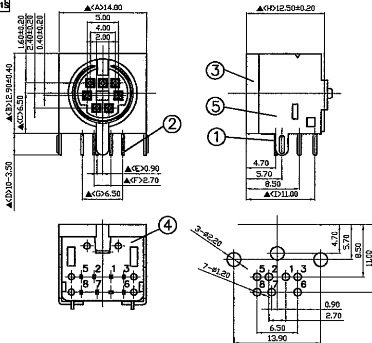
Pin Hole Layout (Jack Bottom View)
