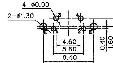
Pin Hole Layout (Jack Bottom View)
