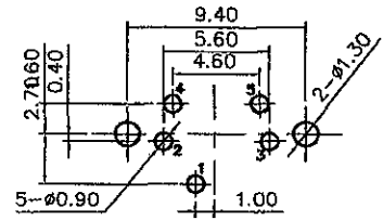
Pin Hole Layout (Jack Bottom View)
