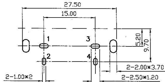
Pin Hole Layout (Jack Bottom View)
