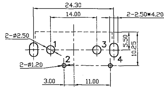
Pin Hole Layout (Jack Bottom View)
