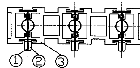
Pin Hole Layout (Jack Bottom View)
