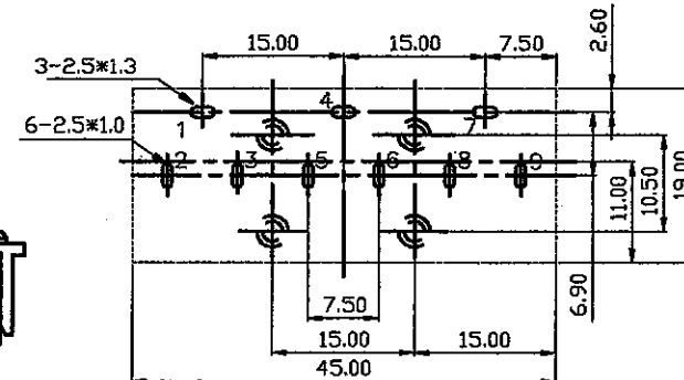
Pin Hole Layout (Jack Bottom View)
