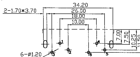
Pin Hole Layout (Jack Bottom View)
