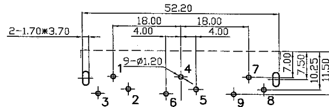
Pin Hole Layout (Jack Bottom View)
