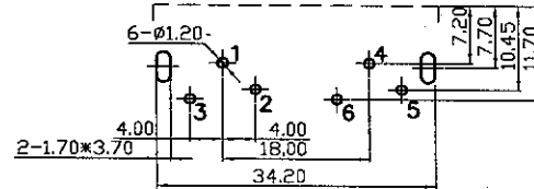
Pin Hole Layout (Jack Bottom View)
