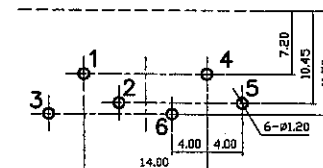
Pin Hole Layout Jack Bottom View
