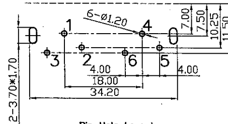
Pin Hole Layout (Jack Bottom View)
