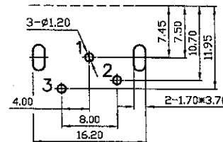
Pin Hole Layout (Jack Bottom View)
