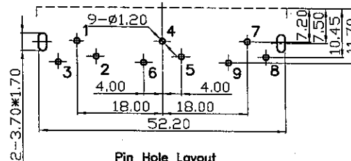
Pin Hole Layout (Jack Bottom View)
