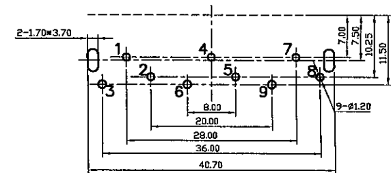
Pin Hole Layout (Jack Bottom View)
